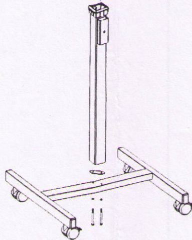
foot installation
