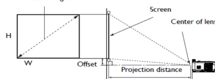
4:3 Screen diagonal
